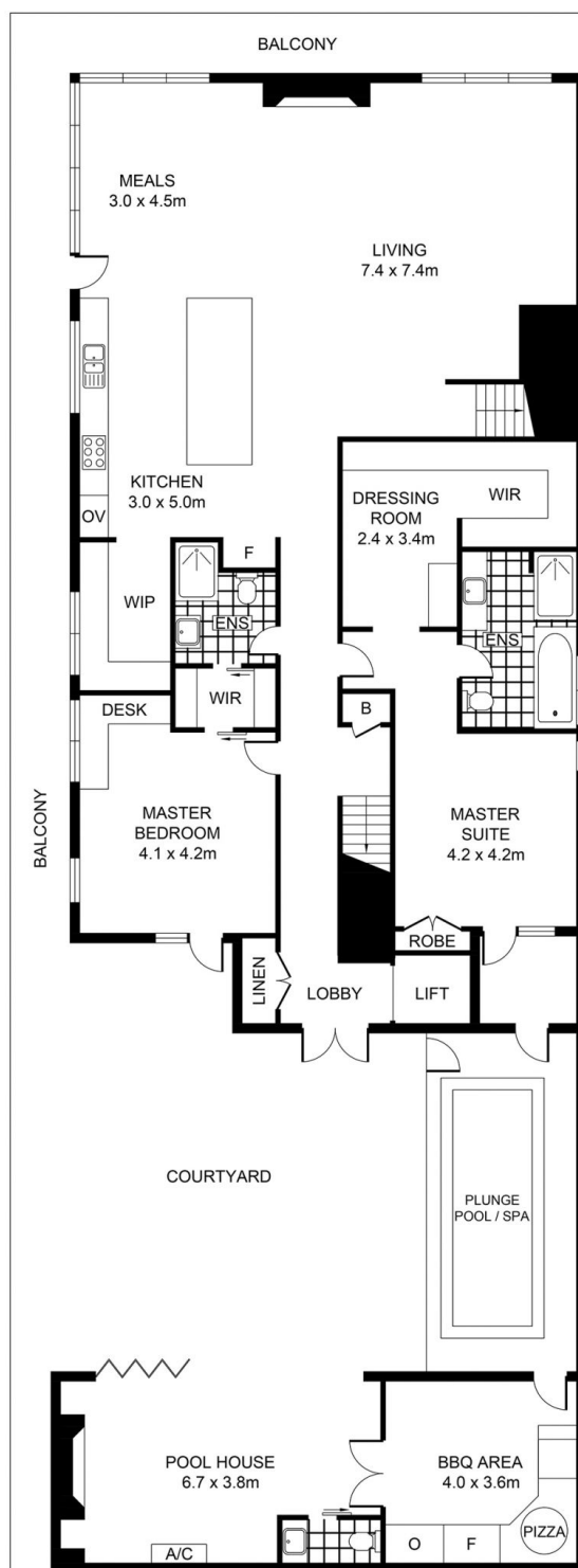
FIRST FLOOR
